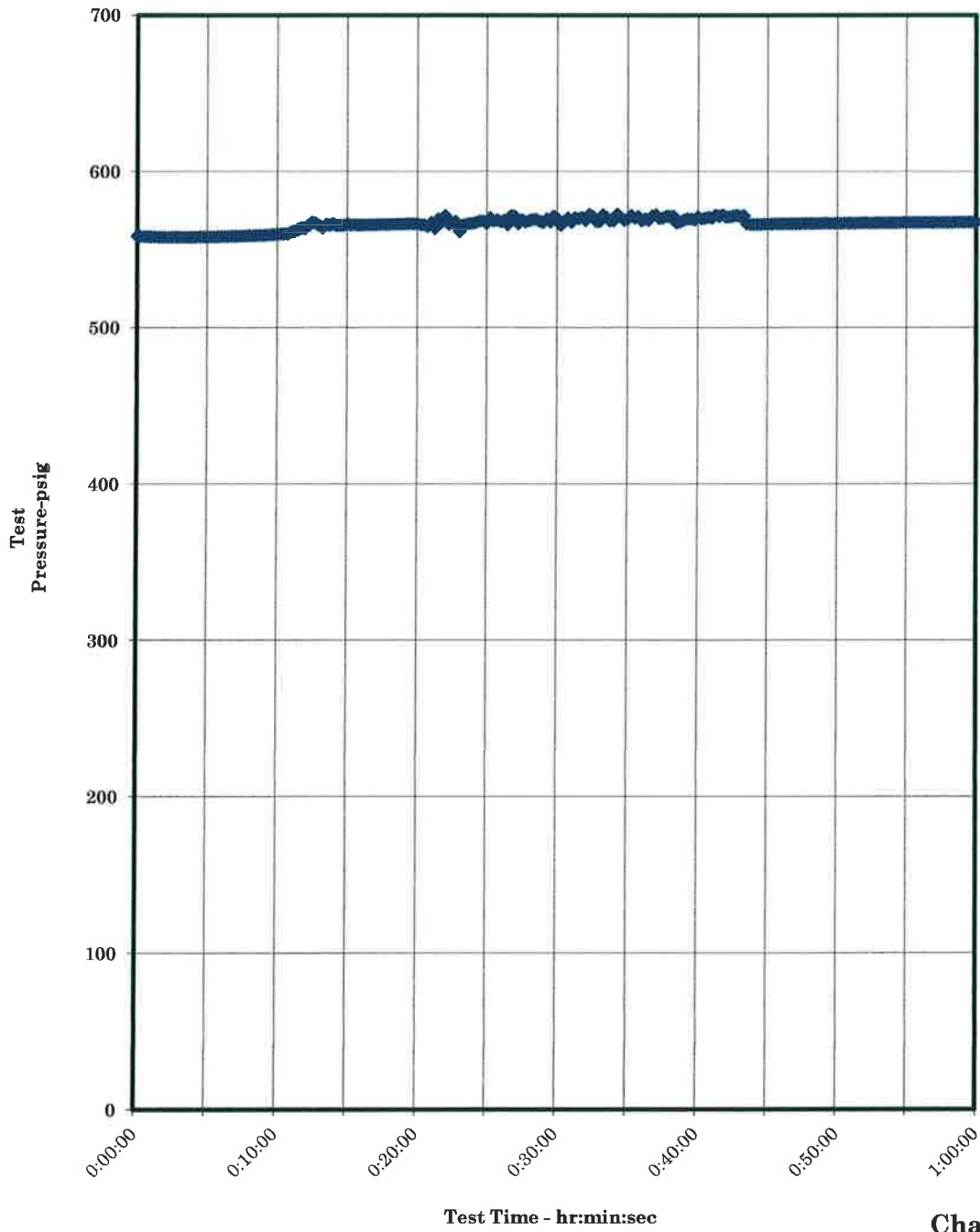
Pressure verses Time Chart
